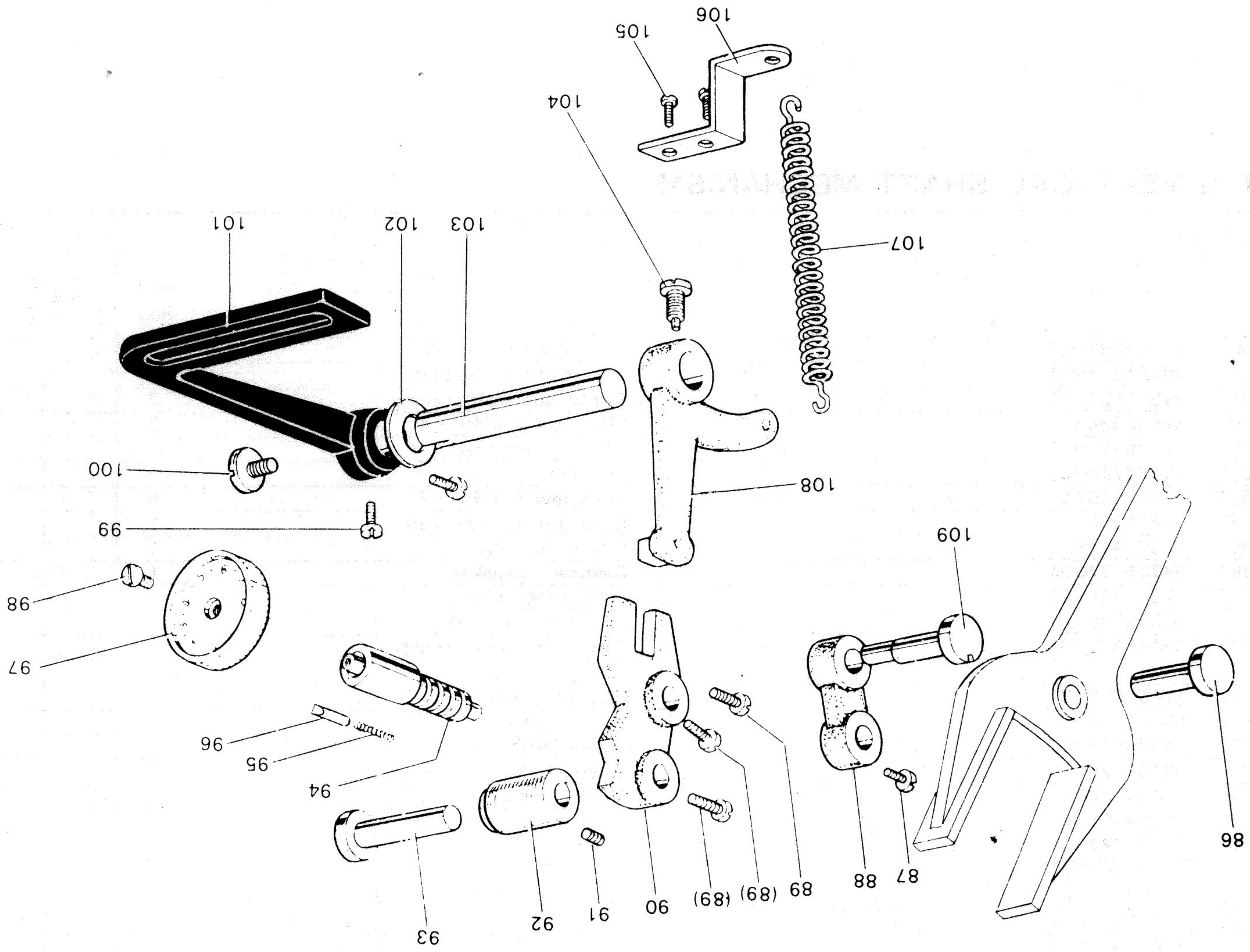
STITCH LENGTH REGULATOR MECHANISM
